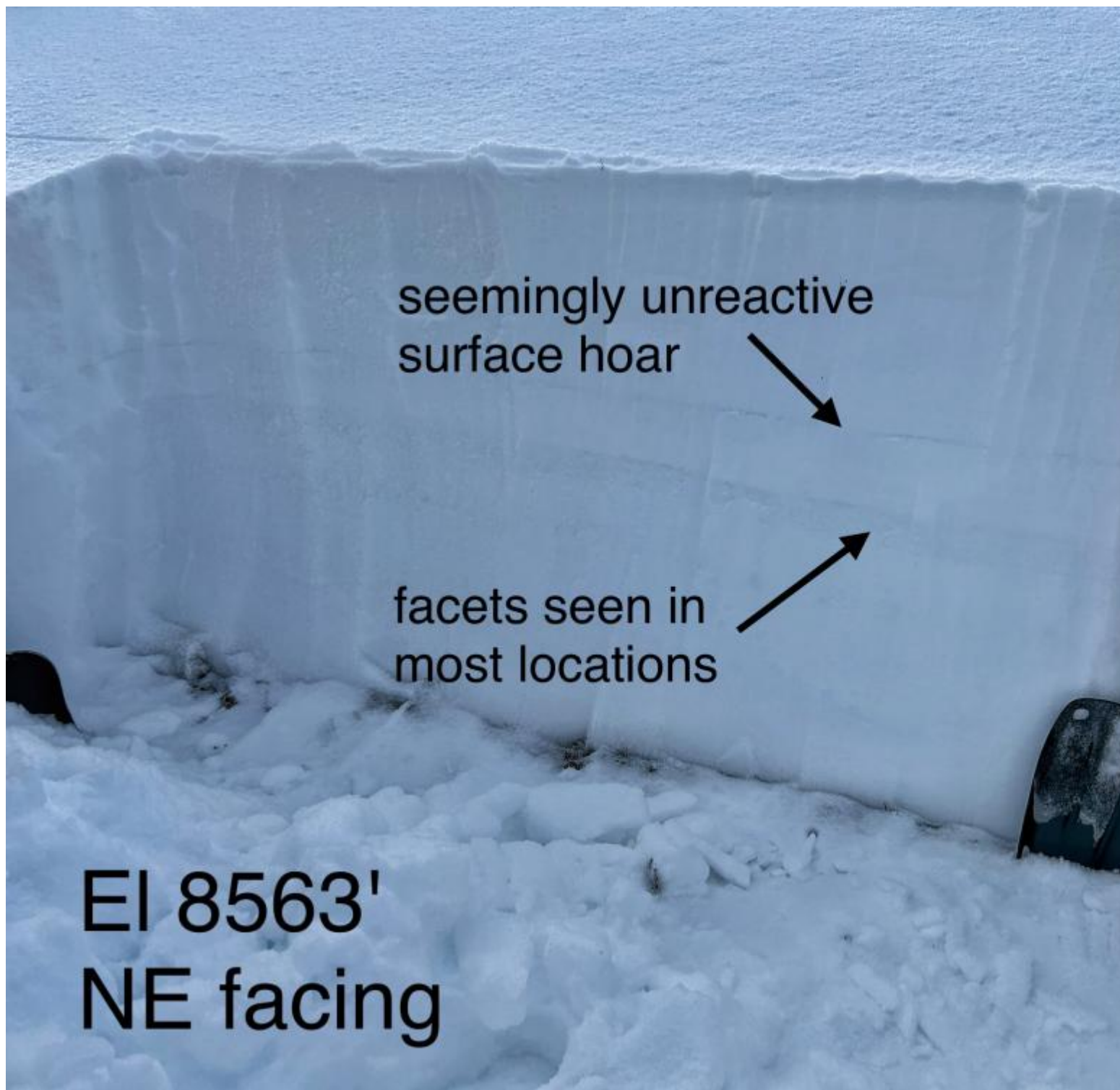
Image of snowpit from just south of the top of the ramp on Dec 22
